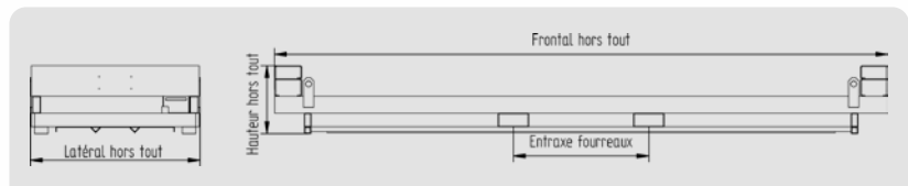
Racks gerbables
